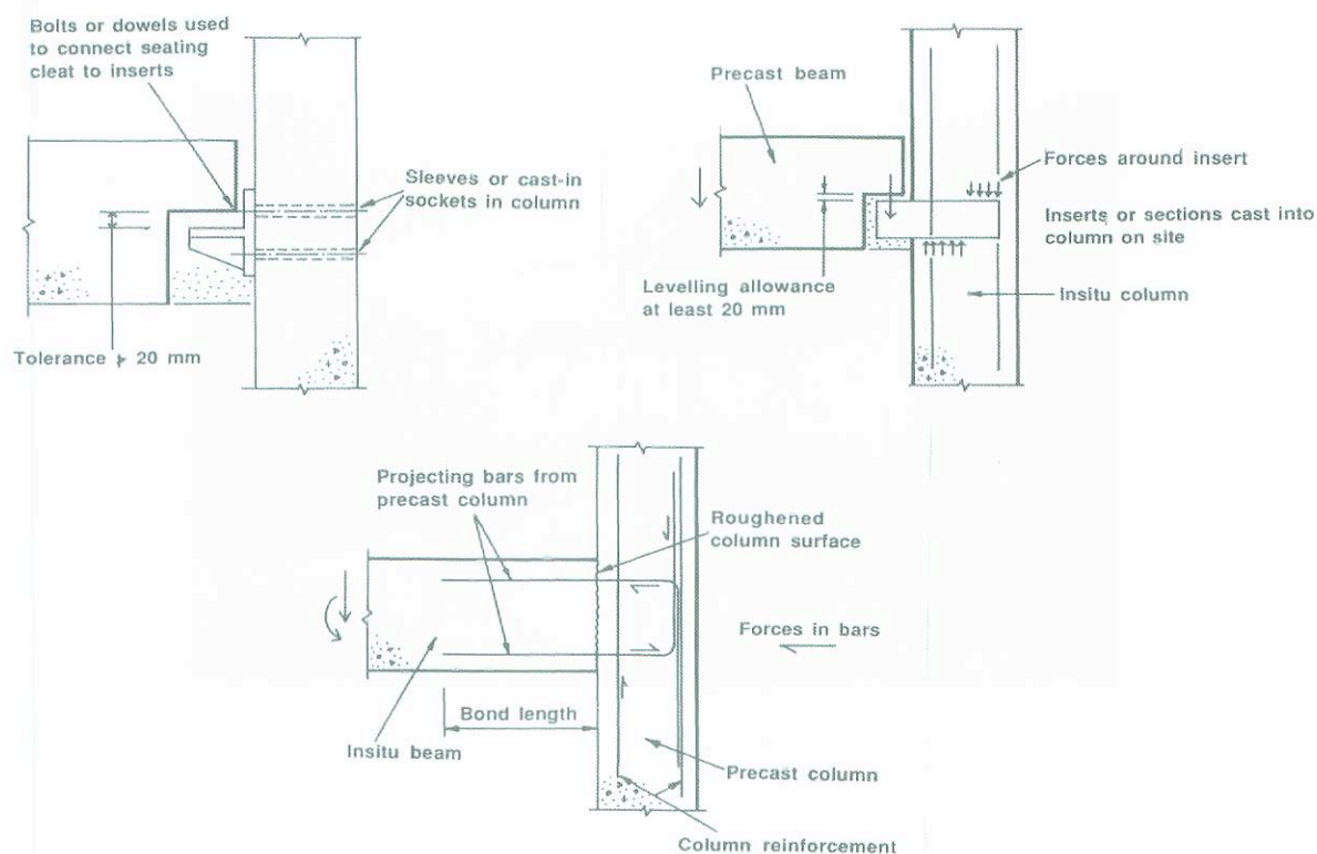
Fig. 2-17: Precast-to-in-situ concrete connection details.
