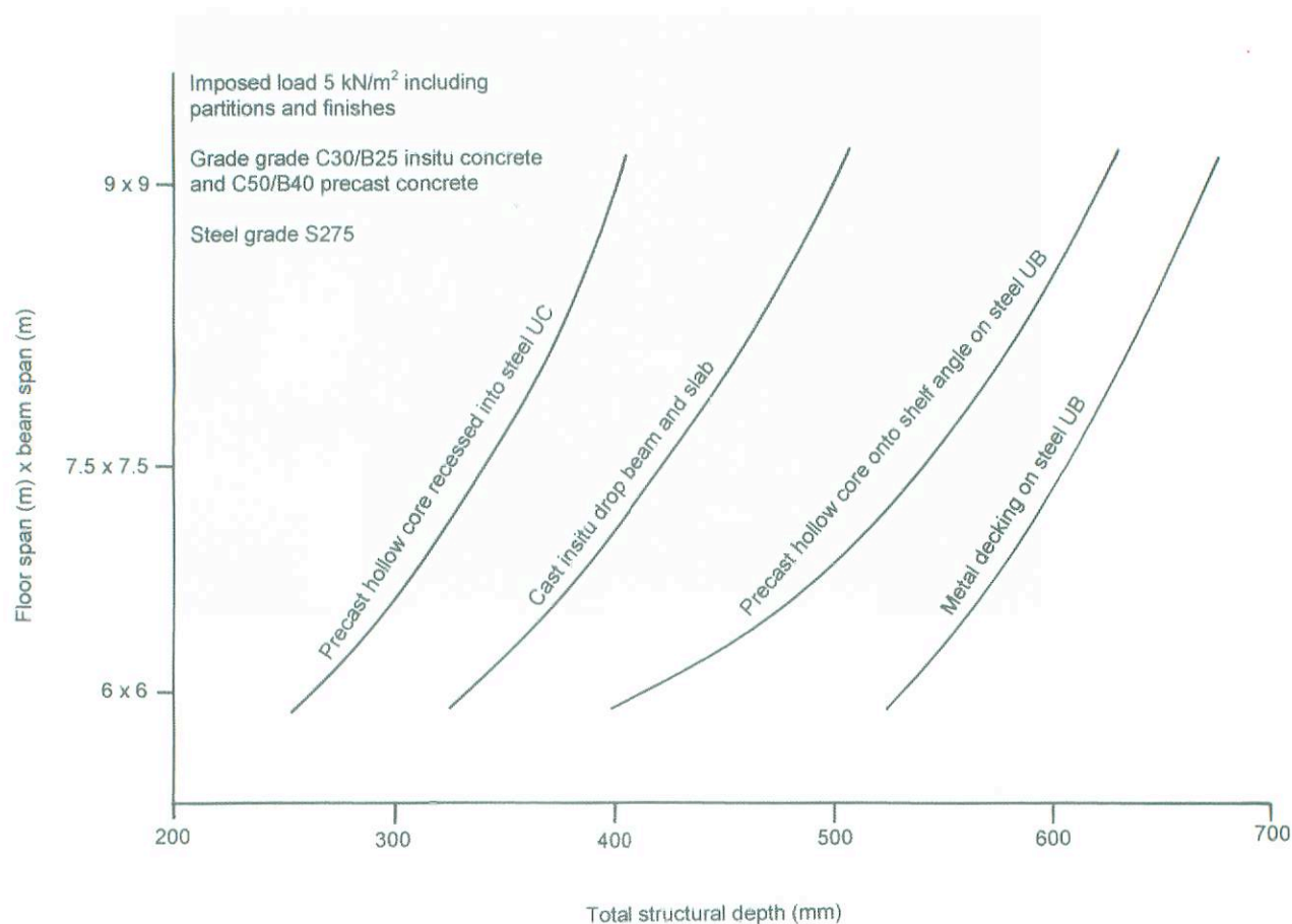
Fig. 1-13: Floor span x beam span data with respect to structural depth.
