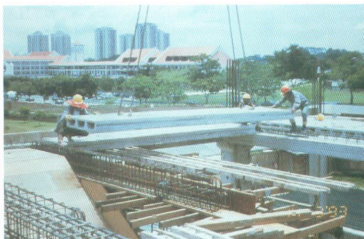
Fig. 2-9: Precast concrete hollow core floors supported on post-cast insitu beams.
