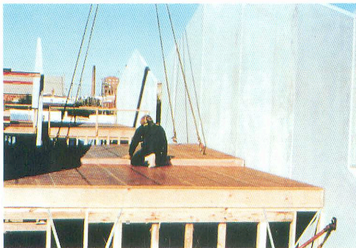
Fig. 4-11: Timber floors and precast concrete walls used for domestic dwellings. (Courtesy C&CA of Australia)
