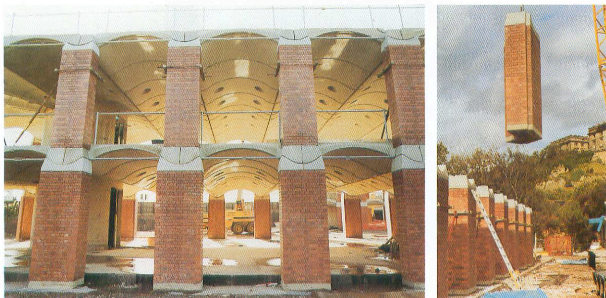
Fig. 1-9: Inland Revenue Building in Nottingham, UK. (Courtesy of Trent Concrete Ltd., UK)
