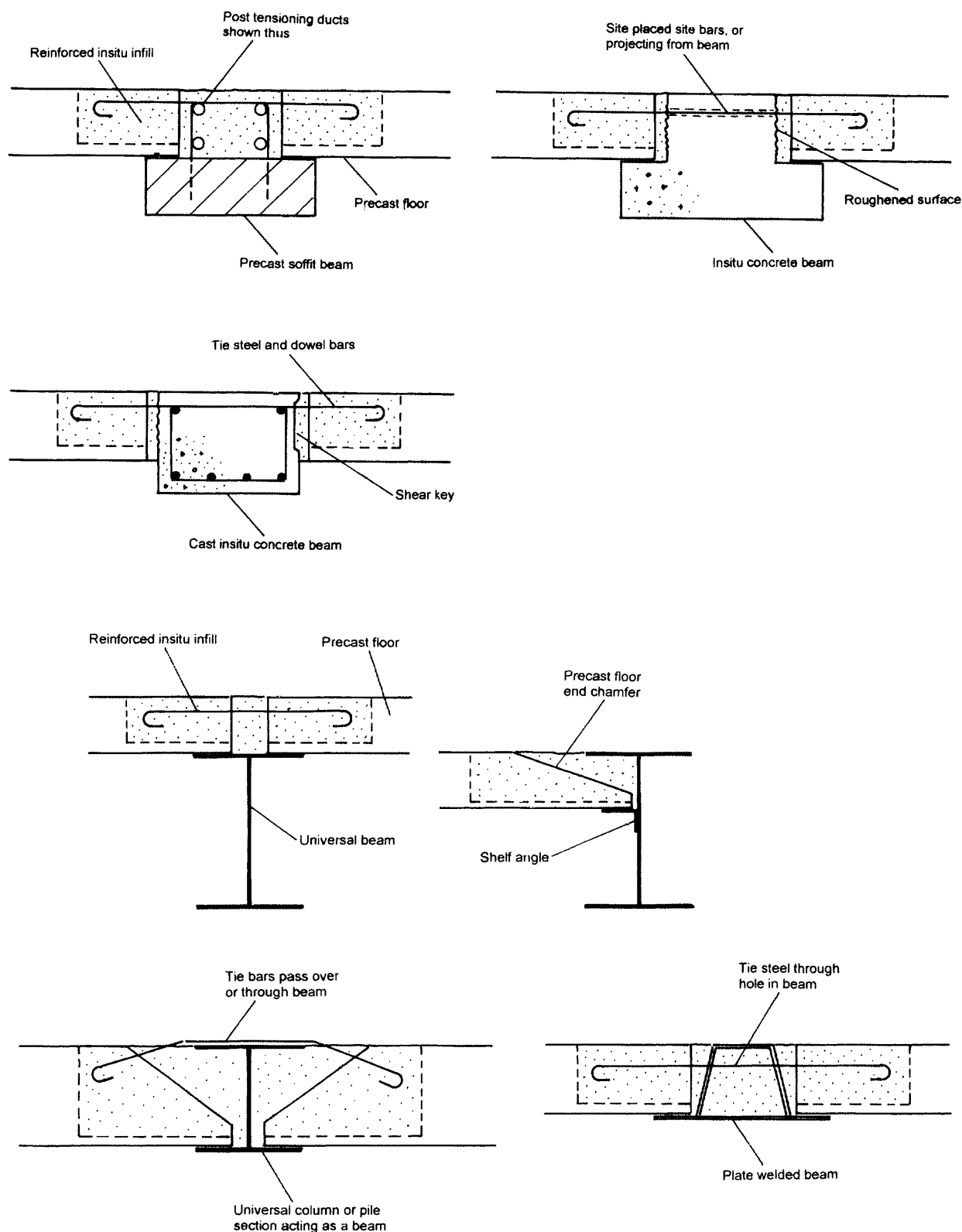
Fig. 1-14: Mixed construction for beams and floor slabs.
