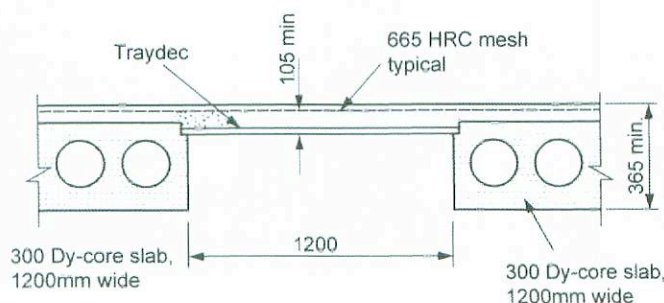
Fig. 3-17: Steel profiled decking spanning between precast hollow core floor units
