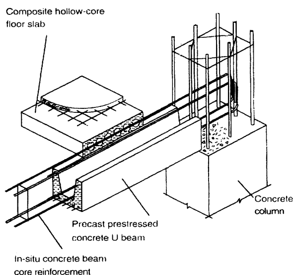
Fig. 2-6: Precast shell beams with cast insitu concrete cores. (Courtesy of Prestressed Concrete Institute, USA)
