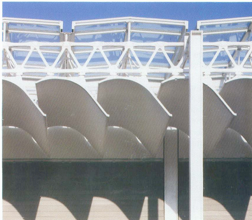
Fig. 1-4: Ferro cement roof structures, working in combination with tubular steel lattices, act as daylight reflectors to a Houston art gallery. (Courtesy of Ove Arup, UK)
