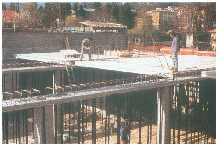
Fig. 2-2: Precast soffit formwork used as permanent shuttering for insitu beams and long span floors. Commercial building in Novara, Italy. (Courtesy of APE and Gruppo Centro Nord, Italy)
