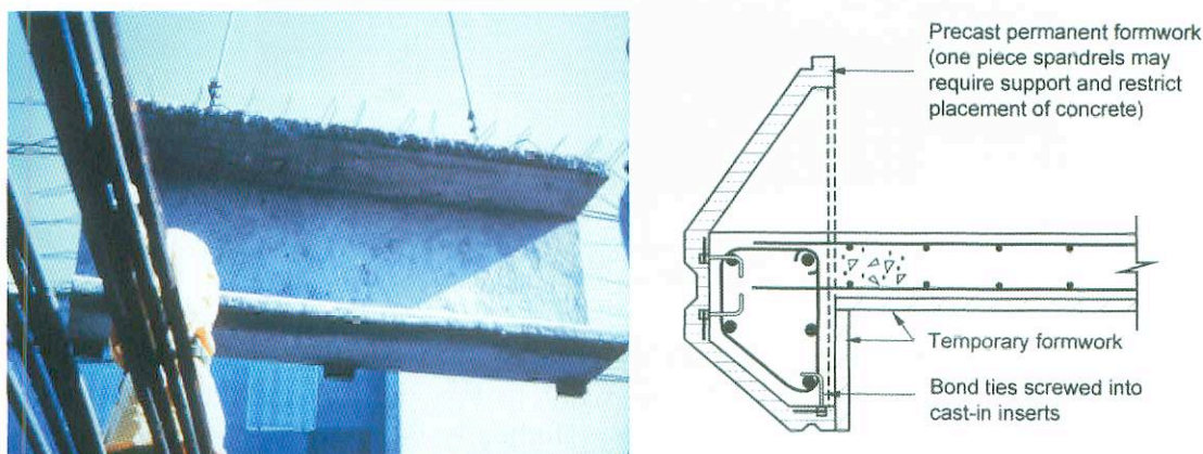
Fig. 2-1: Precast permanent shuttering for cast insitu concrete floors at City Corp Centre, Sao Paulo. (Courtesy of Mario Franco, Brazil, left, and Reinforced Concrete Council, UK, right)
