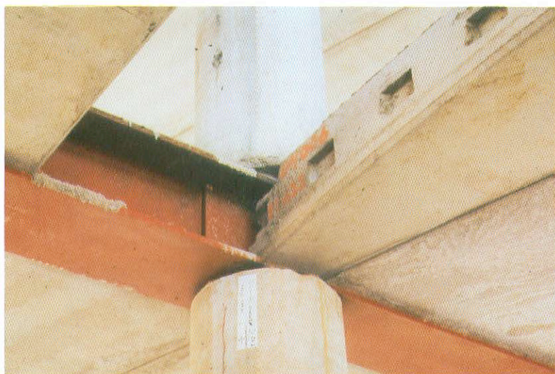
Fig. 3-4: Precast floors supported on the bottom flanges of rolled steel Universal beams or column sections. (Courtesy of Strängbetong, Sweden)
