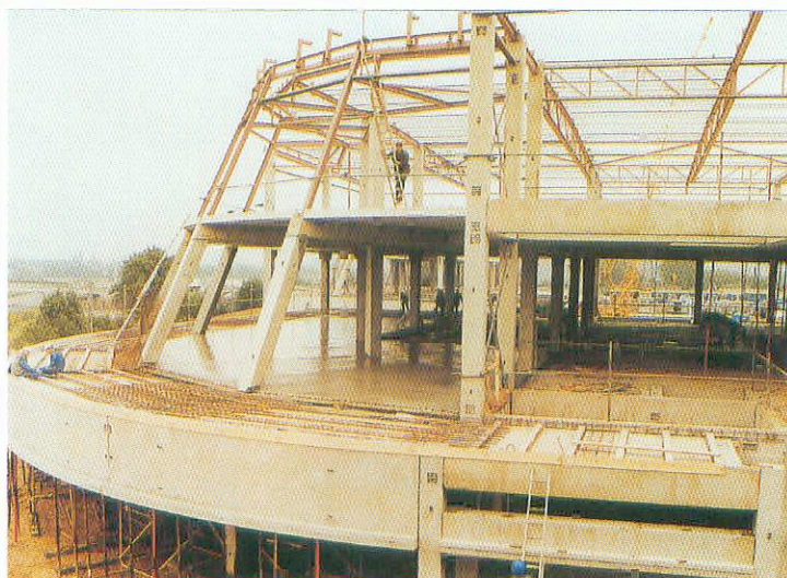
Fig. 3-23: Steel mansard roof on to a precast concrete frame (Courtesy of Composite Structures, UK)
