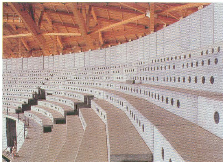
Fig. 4-2: Glue laminated timber space truss provides the roof to a precast structure at Lisbon's Expo '98 site. (Courtesy Prêgaia, Portugal)
