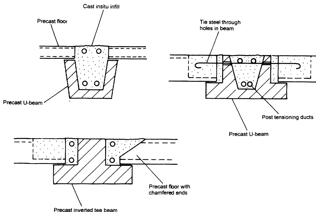
Fig. 2-5: Precast beams awaiting infill concrete and post-tensioning [top] in the trough of U-beams [bottom] to the side of inverted tee beams.
