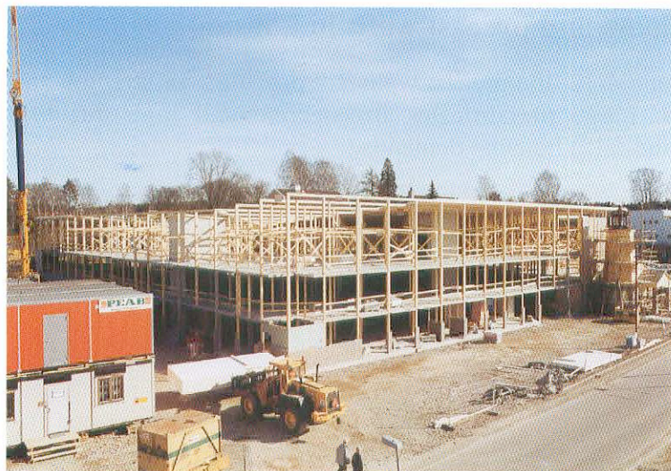
Fig. 4-8: Glue laminated timber beams and columns support precast flooring in a warehouse (Courtesy of Strängbetong, Sweden)
