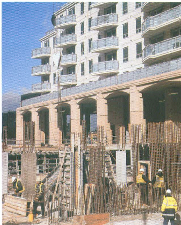
Fig. 2-20: Precast cladding on cast insitu frame - 750 apartments at St George Wharf, London. (Courtesy of Thomas Telford Ltd., London)
