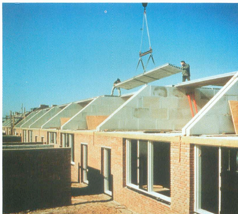
Fig. 5-5: Precast partition walls and load bearing brickwork support precast hollow cored floor units in low rise dwellings (Courtesy of VBI, Netherlands)
