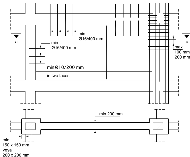
Fig. 11: Co-axial shear wall
