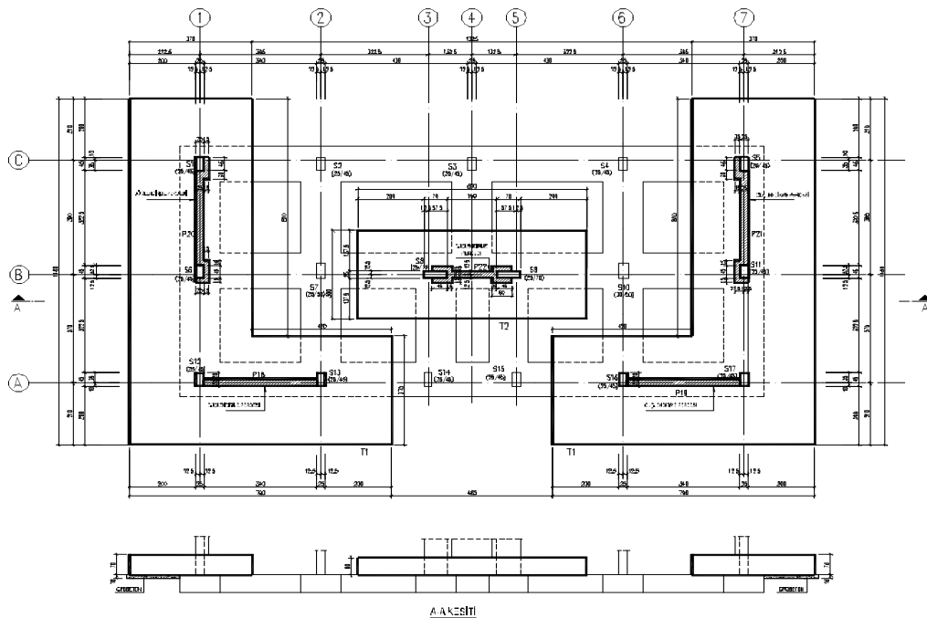
Fig. 16: Foundation layout for the new shear walls
