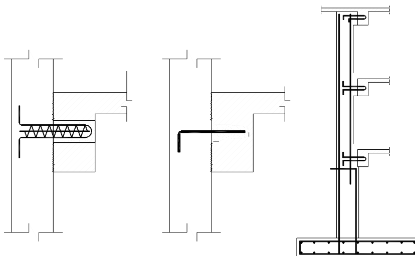
Fig. 12: Added external shear wall
