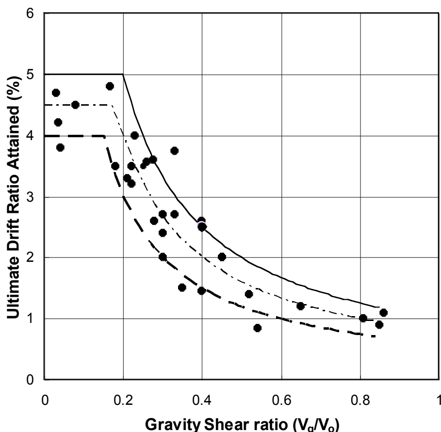
Fig. 7 Effect of gravity shear ratio on ultimate drift capacity (Dots are experimental points, lines are bounds for the experiments)
