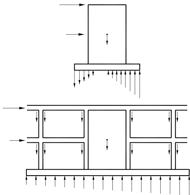
Fig. 10: Added shear wall and its foundation
