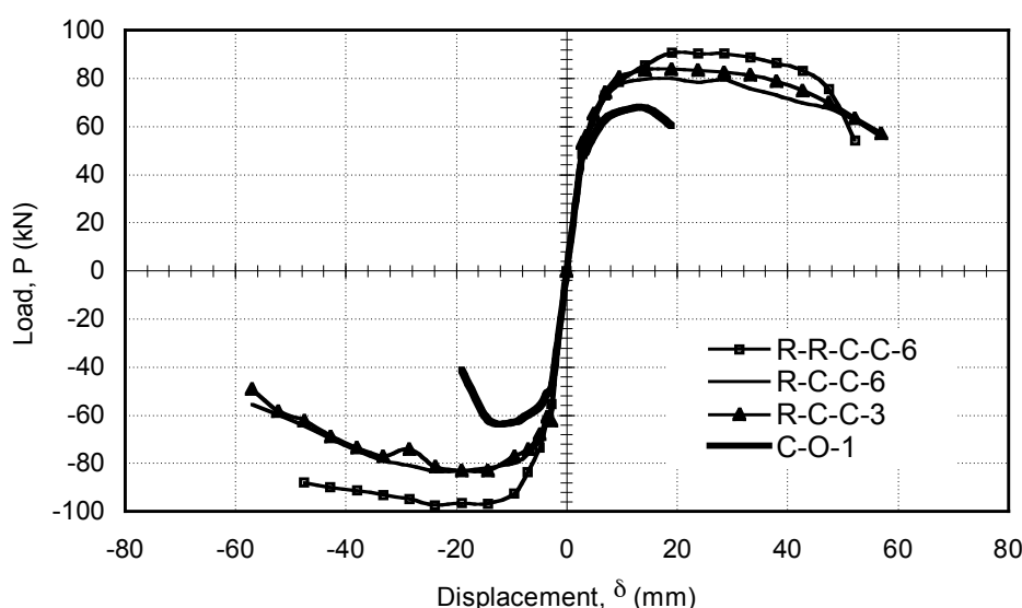
Fig. 20: Envelopes of load-displacement relationships (Ilki et. al 2004)
