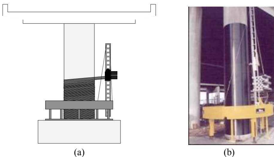
Fig. 4: Automated RC column wrapping. (a) Schematic. (b) Photograph of robot-wrapper.
