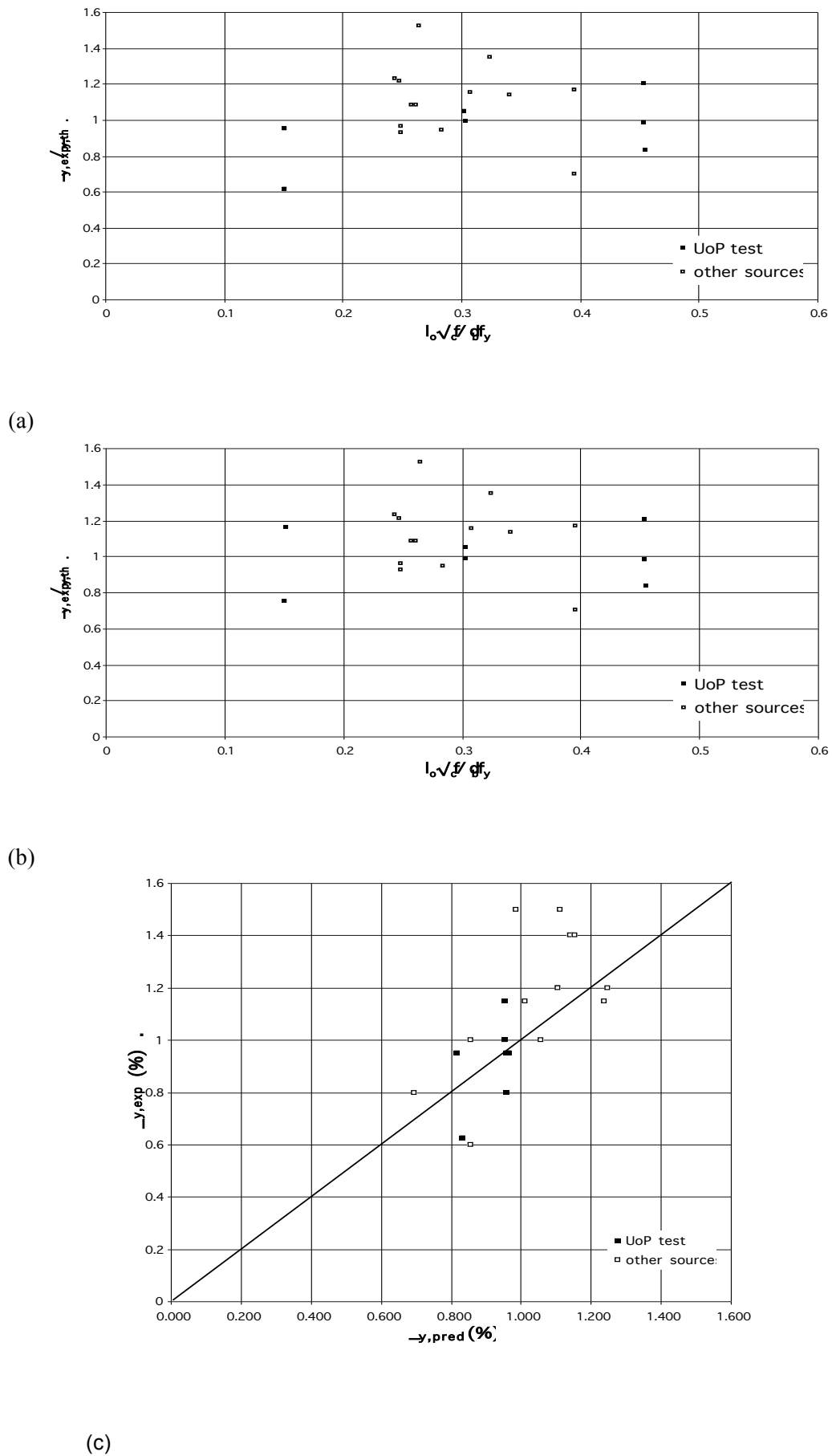
Fig. 10: Comparison of experimental \theta_y of members with lap-spliced ribbed bars and FRP wrapping to value predicted: (a) without, or (b), (c) with the correction for the effect of lap splicing.
