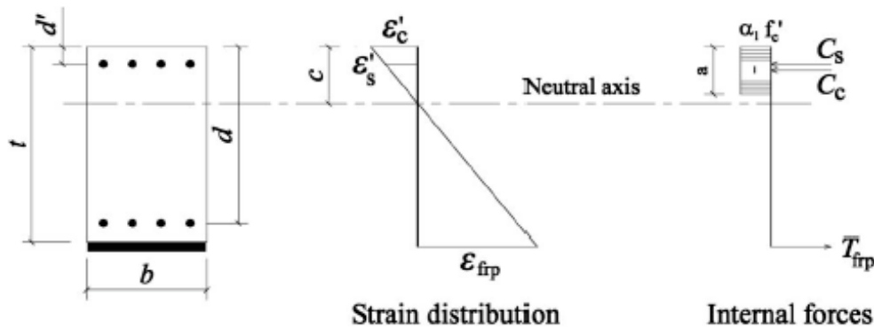
Fig. 23: Determination of the required number of FRP laminates
