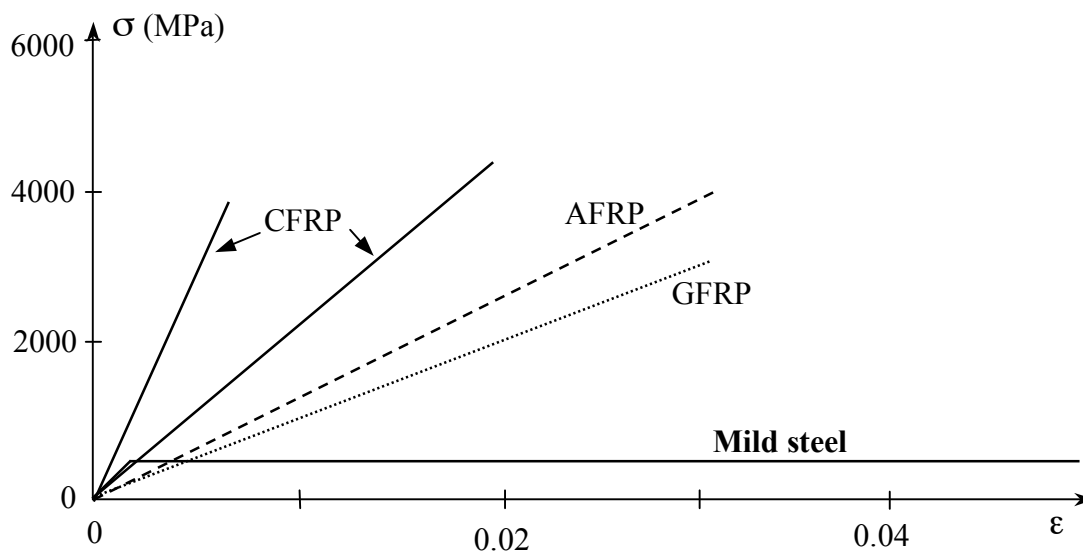
Fig. 1: Uniaxial tension stress-strain diagrams for different unidirectional FRPs and steel. CFRP = carbon FRP, AFRP = aramid FRP, GFRP = glass FRP.
