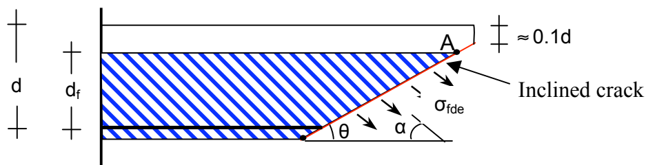
Fig. 21: Contribution of composite materials to shear resistance.
