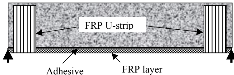
Fig. 2: Strengthened RC beam with FRP U-strip
