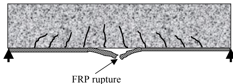
Fig. 3: Flexural failure
