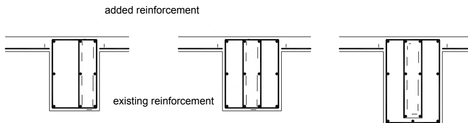
Fig. 6: Jacketing of beams
