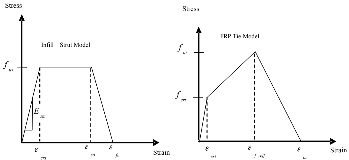
Fig. 21: Stress-strain behaviour of the infill strut and FRP tie
