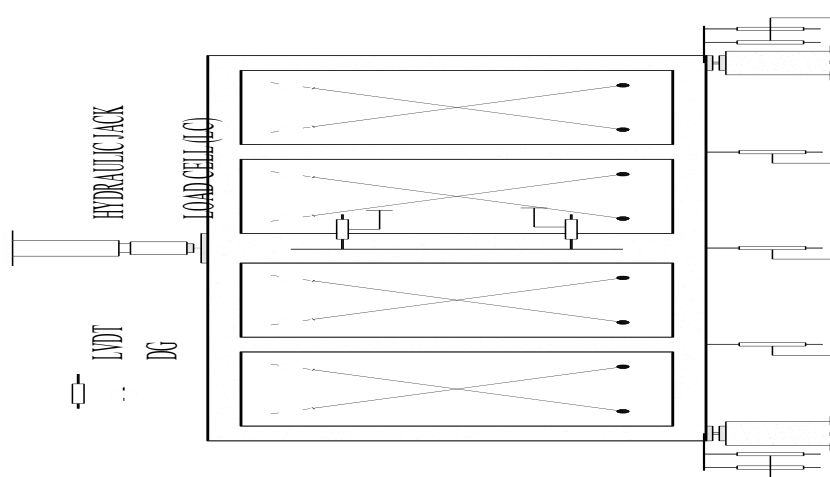
Fig. 6: Instrumentation
