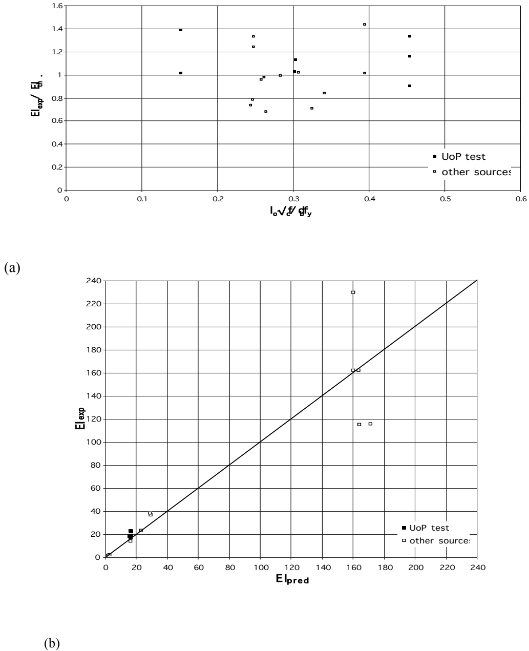
Fig. 11: Comparison of experimental EI_{eff} = M_y L_s / 3 \theta_y of members with lap-spliced ribbed bars to value predicted after correction of M_y , \theta_y for the effect of lap splicing according to the rules in 2.3.2.
