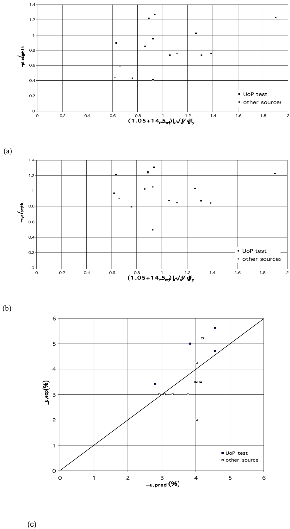
Fig. 12: Comparison of experimental \theta_u of members with lap-spliced ribbed bars and FRP wraps to the value predicted: (a) without, or (b), (c) with the correction for the effect of lap splicing.
