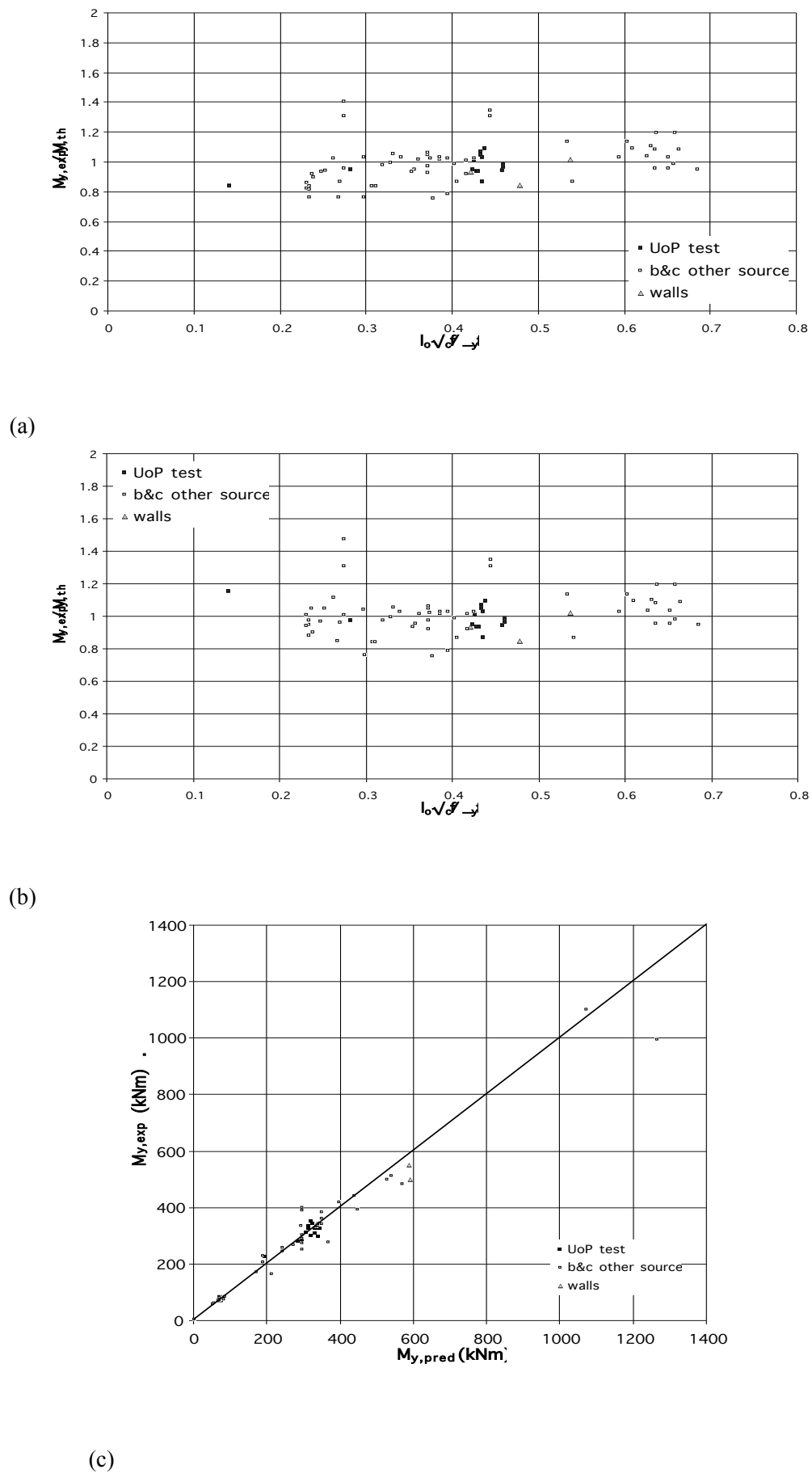
Fig. 1: Comparison of experimental M_y of members with lap-spliced ribbed bars to value predicted: (a) without, or (b), (c) with the correction according to the rules in 2.2.2.
