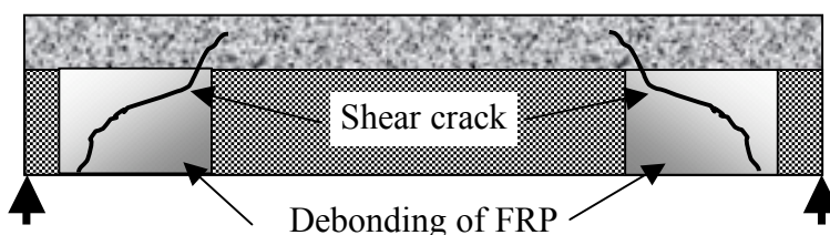
Fig. 7: Shear failure due to FRP debonding
