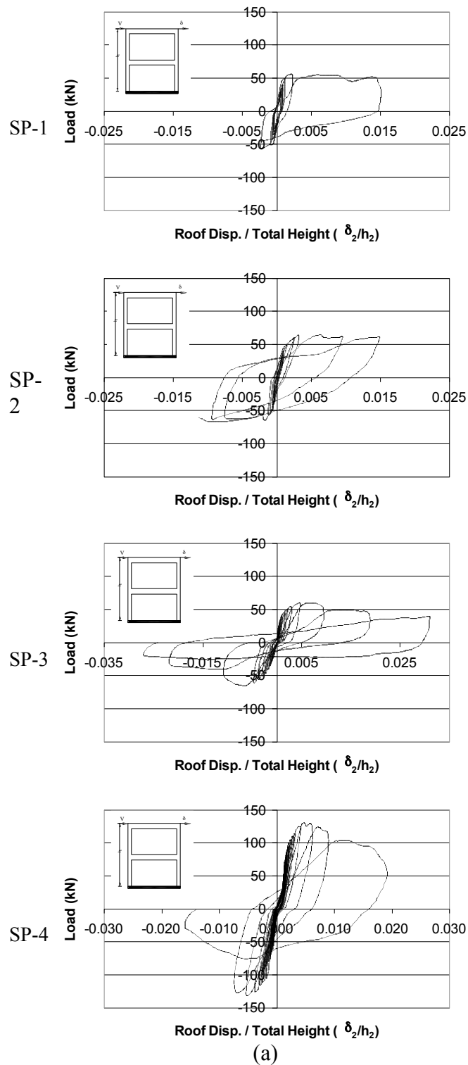
Fig. 7: (a) Lateral load vs. roof drift ratio hysteretic relationships for all test specimens; (b) specimens at the end of the test.
