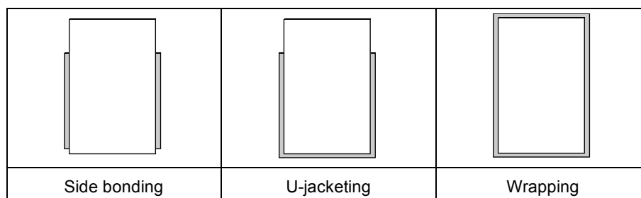
Fig.8: FRP shear strengthening configurations on the cross-section.
