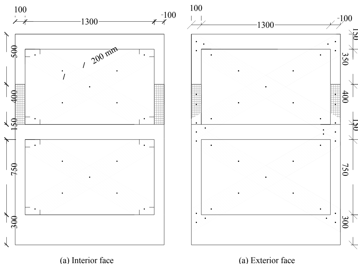
Fig. 4: CFRP arrangement and location of the anchor dowels in Specimen SP-5 (dimensions are in mm)
