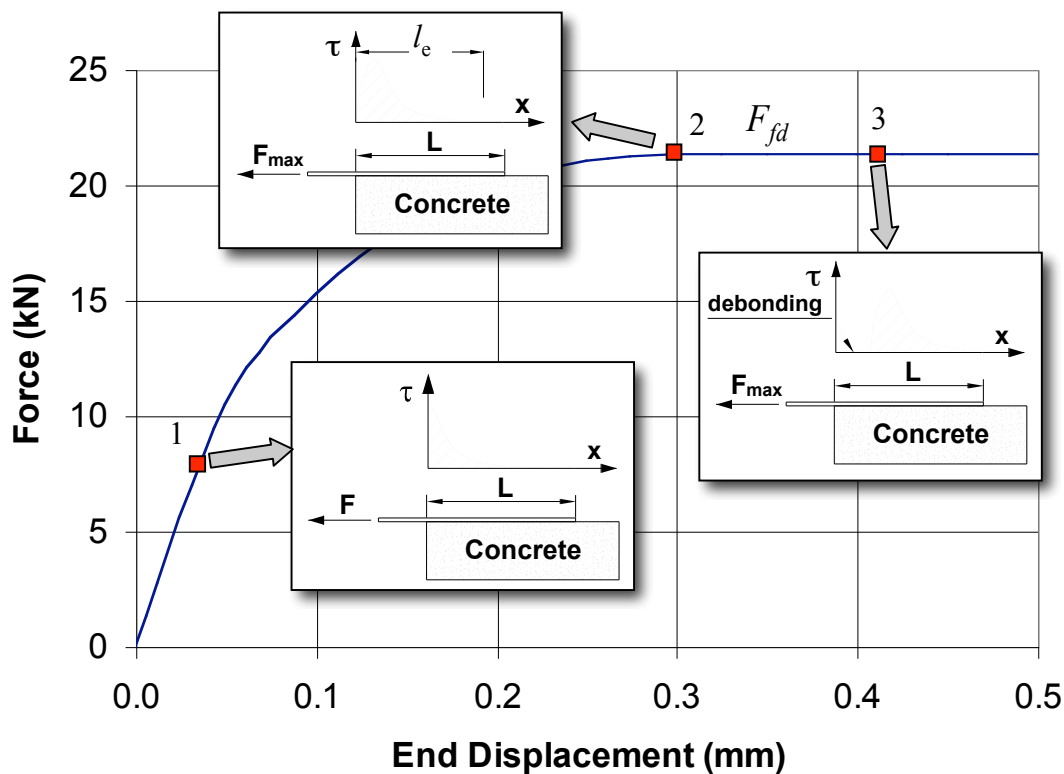
Fig. 1: Force-slip response of the example anchored FRP sheet, with characteristic points and corresponding bond fields.
