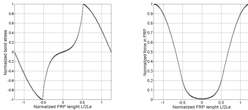
Fig.3: ULS: (a) Bond stress along the FRP; (b) Force along the FRP for s_{rm} \geq 2l_e .
