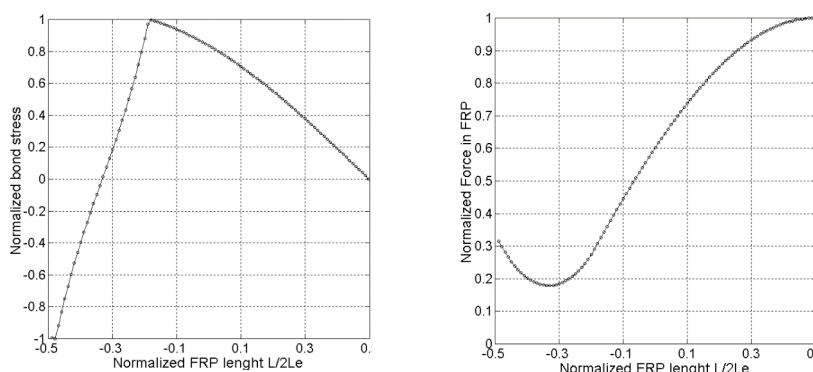
Fig. 6: Same as Fig. 4, in a variable bending moment zone.
