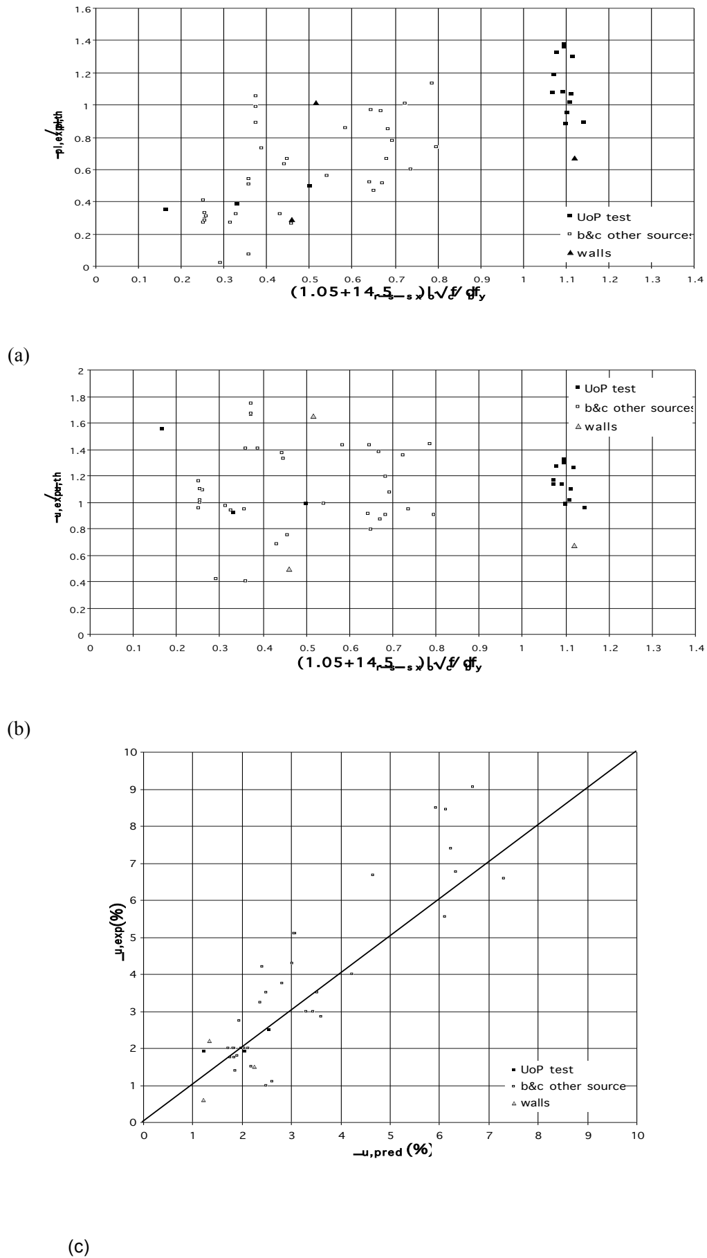
Fig. 4: Comparison of experimental \theta_u of members with lap-spliced ribbed bars to value predicted: (a) without, or (b), (c) with the correction according to the rules in 2.2.2.
