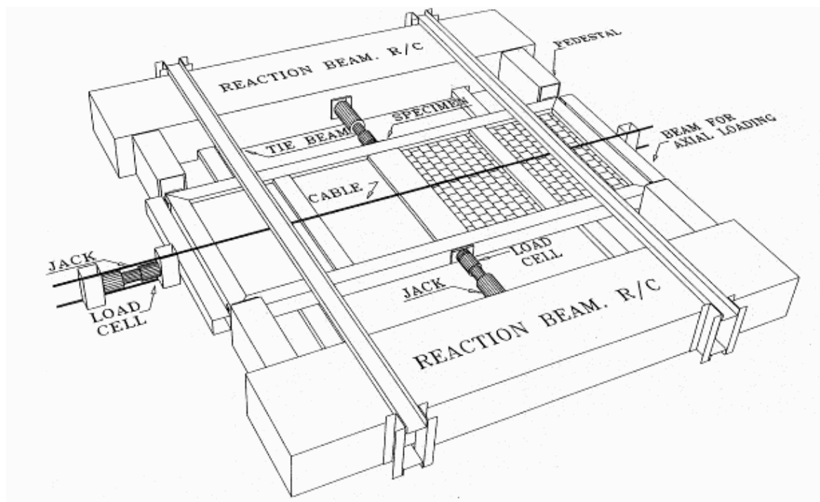
Fig. 5: Test Set-Up
