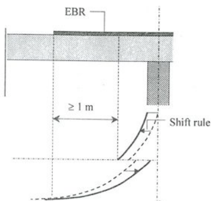
Fig.2: Anchorage above internal supports ( fib Bulletin 14 )
