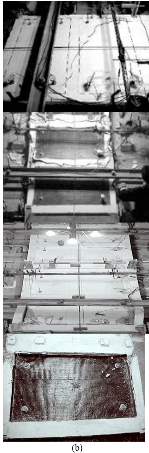
Fig. 7: (a) Lateral load vs. roof drift ratio hysteretic relationships for all test specimens; (b) specimens at the end of the test.
