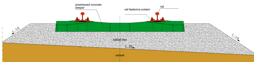
Figure 2-1: Ballasted track
