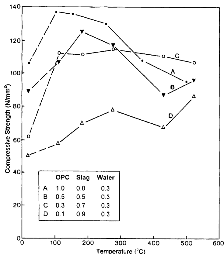
Figure 3.20: Improvement of the temperature function of strength of OPC paste with the addition of slag [KHO 92]
