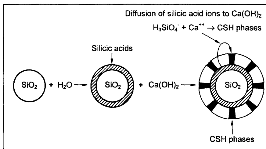
Figure 3.18. Schematic presentation of the hydrothermal reaction between reactive silica ( \text{SiO}_2 ) and \text{Ca(OH)}_2 [KOT 79]
