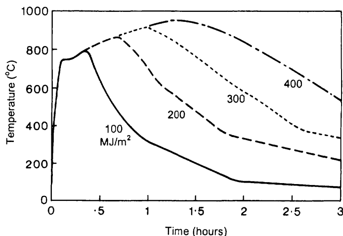
Figure 1.4: Time temperature development of natural (parametric) fires with cooling branches for heat loads ranging from 100 to 400 \text{ MJ/m}^2 and an opening factor of 0.04 \text{ m}^{0.5} [MAG 70].
