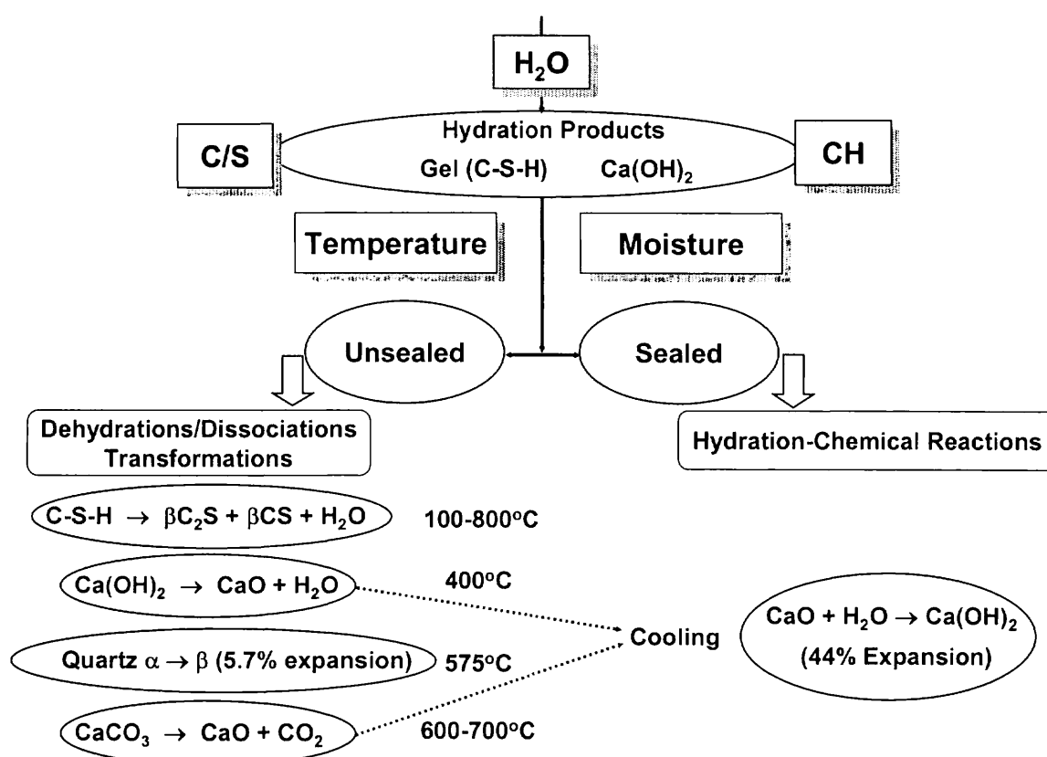
Figure 3.5: The influence of temperature and moisture (sealed and unsealed) upon the chemical transformation of hydration products [KHO-05].
