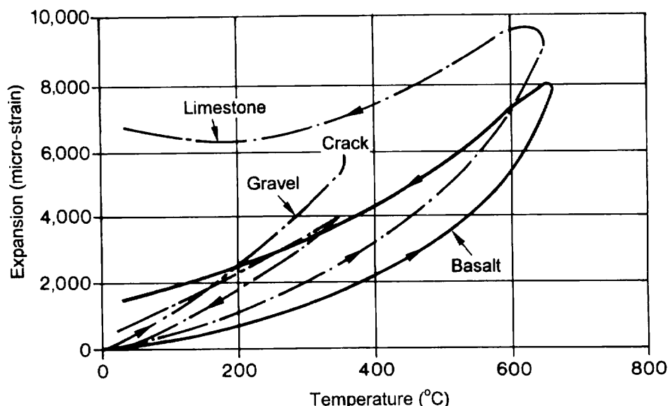
Figure 3.15: Thermal strain during the first heat cycle (2°C/min) of three rectangular aggregates (20-30mm) showing the break-up of Thames river gravel at 350°C, and the lower thermal stability of the limestone than the basalt [KHO 85b]
