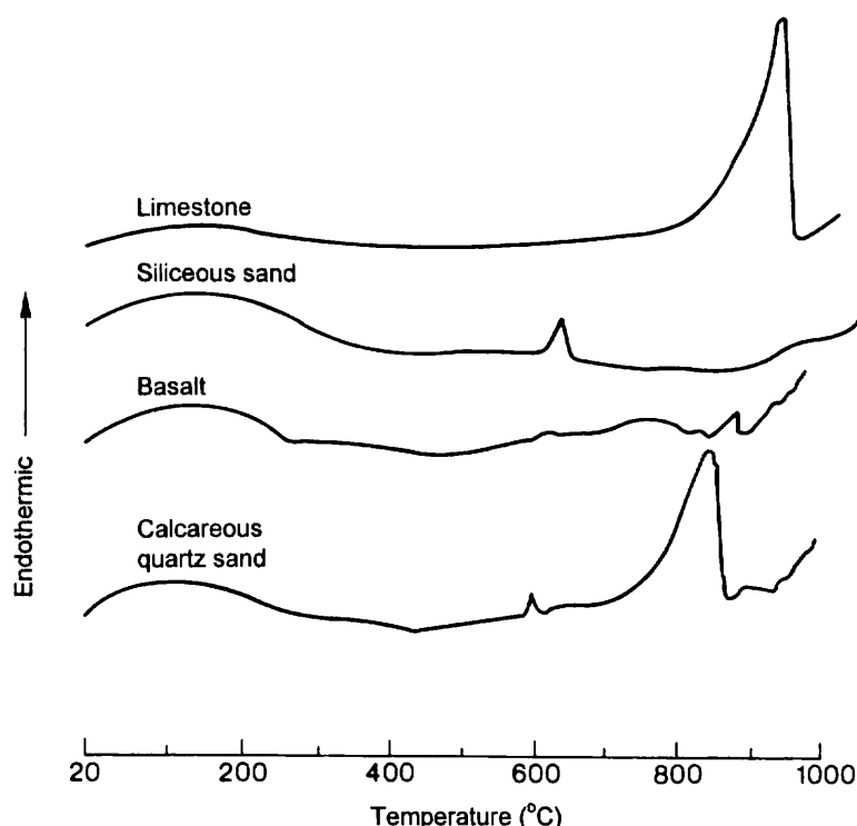
Figure 3.14: Physico-chemical transformations in four different aggregates as measured by DTA during heating at 10°C/min in nitrogen [KHO 85b]
