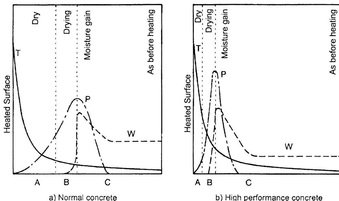
Figure 3.4: Schematic diagram showing temperature ( T ), moisture ( W ) and pore pressure ( P ) states during heating in "normal" and "high strength" concrete.
