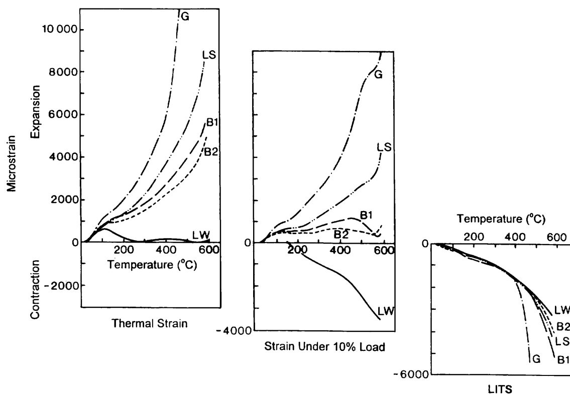
Figure 5.3: Thermal strains of 5 concretes measured during first heating (from the initially air dry condition) at 1^{\circ}\text{C}/\text{minute} under 0% (TS) and 10% load. The "Master" LITS (similar to the 5 concretes up to about 450^{\circ}\text{C} ) is determined as the contraction strain measured between the loaded and the unloaded specimens.
