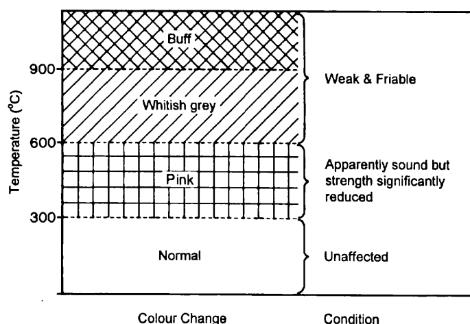
Figure 3.21: Colour changes in heated siliceous concrete.
