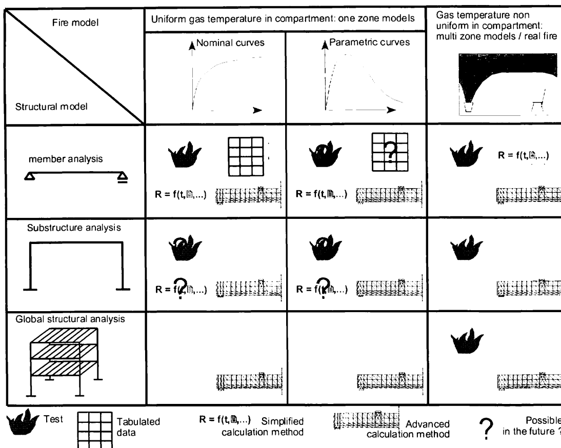
Figure 2.3: Overview of fire assessment methods for increasing complexity of fire and structural models.
